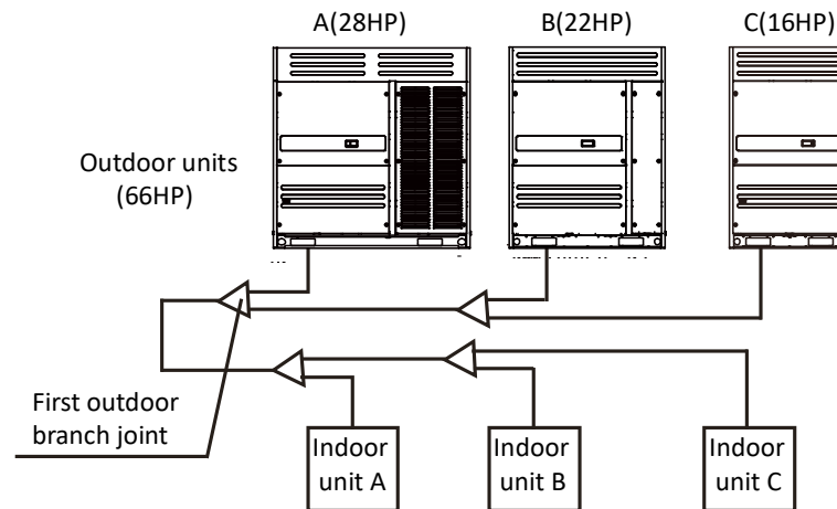
Figure 3-2.4: Positioning of master and slave units
