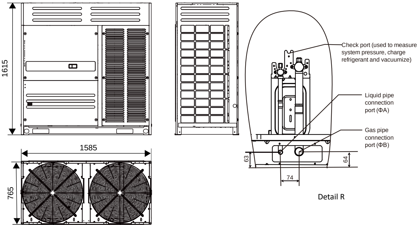
Figure 2-2.3: 24/26/28/30HP dimensions (unit: mm)
