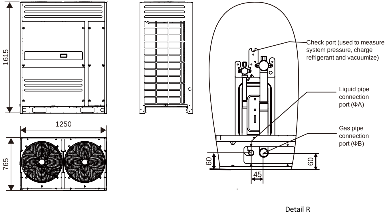
Figure 2-2.2: 18/20/22HP dimensions (unit: mm)
