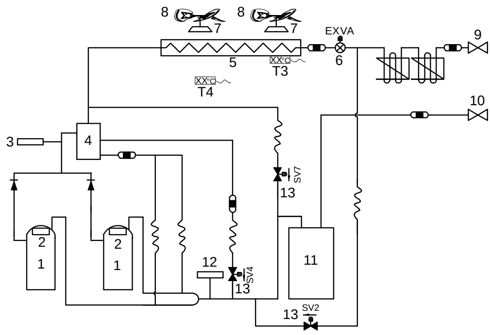
Figure 2-4.2: 18-22HP piping diagram
