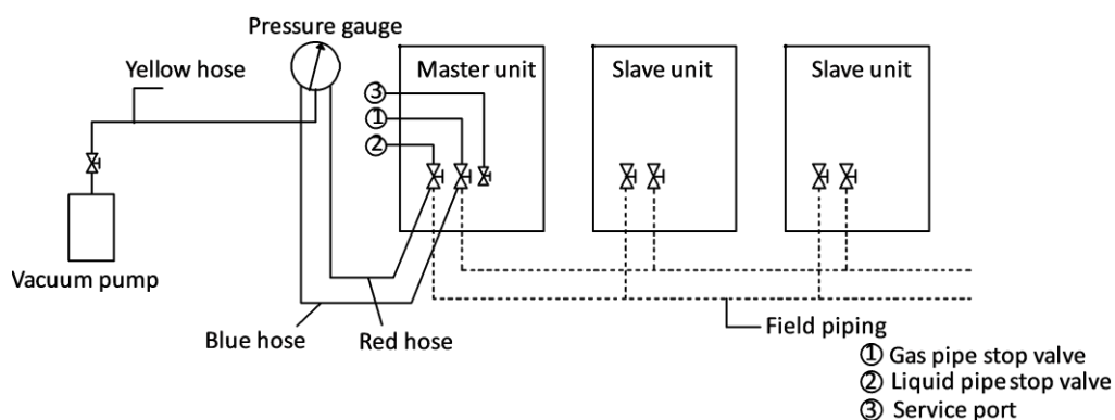
Figure 3-5.14: Vacuum drying
