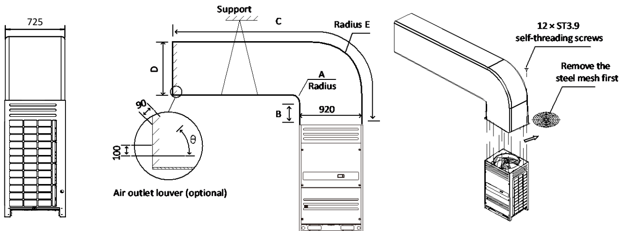
Figure 3-3.3: Longitudinal ducting for 8-16HP units (unit: mm)
