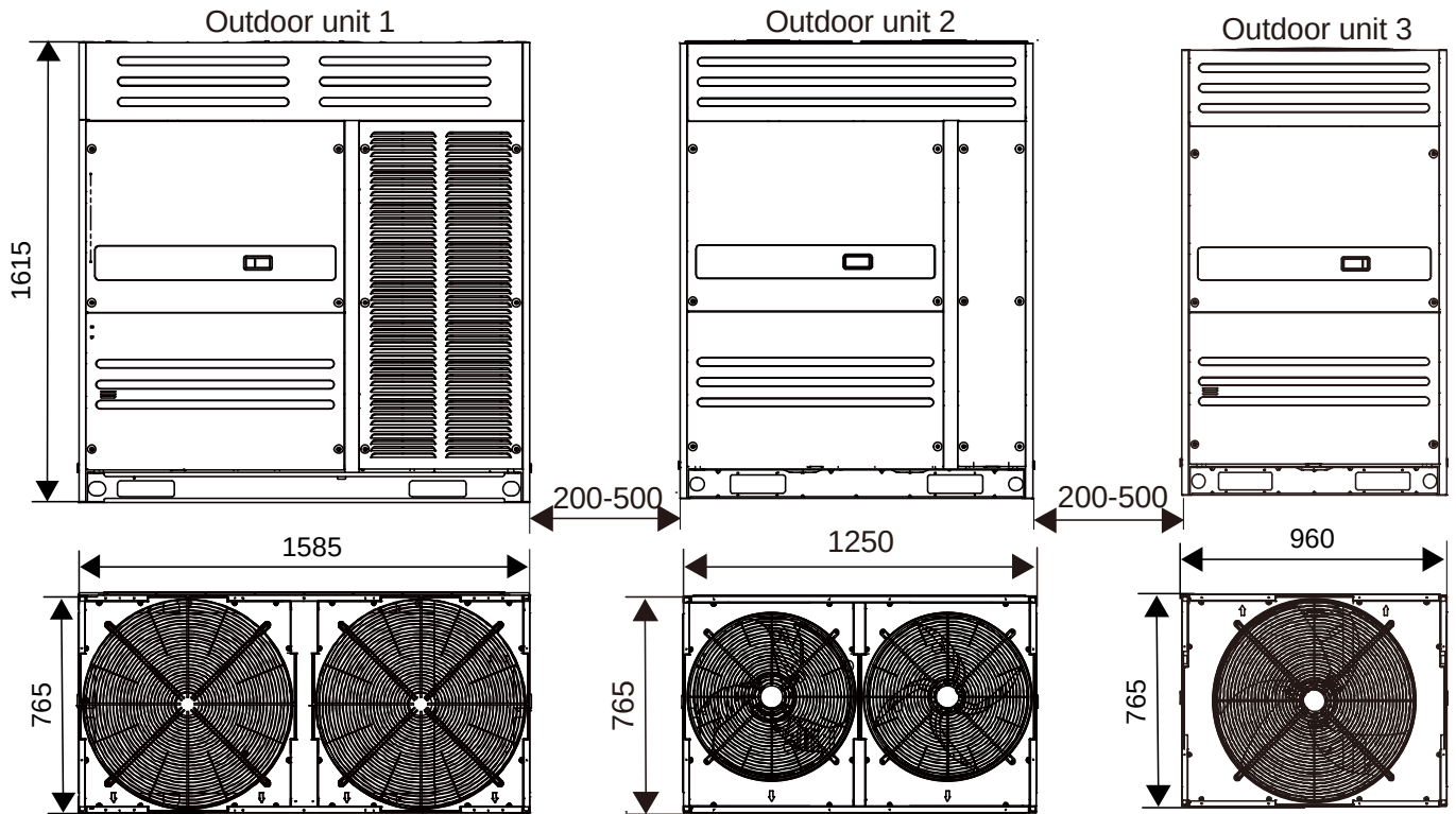
Figure 2-2.10: 64/66/68HP dimensions (unit: mm)
