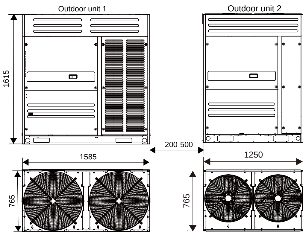
48/50/52HP Figure 2-2.7: 48/50/52HP dimensions (unit: mm)
