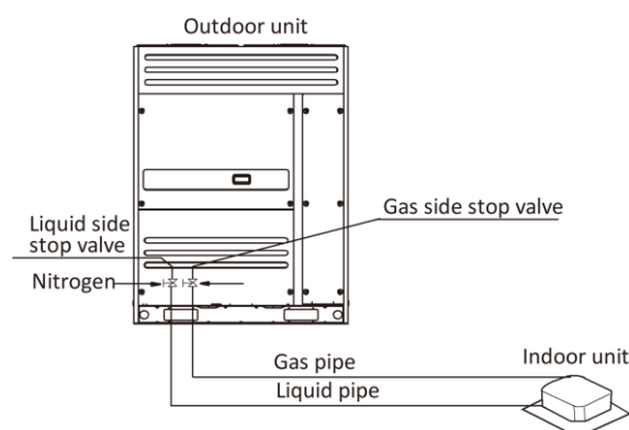
Figure 3-5.13: Gastightness test
