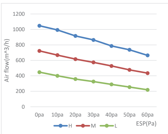
MKT4-500FG50-CL
