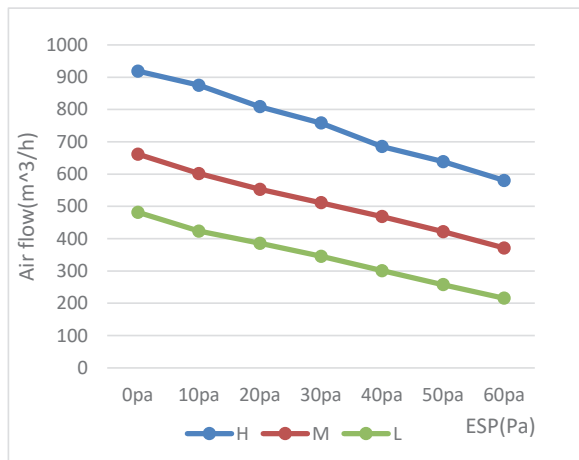
MKT4-400FG50-CL
