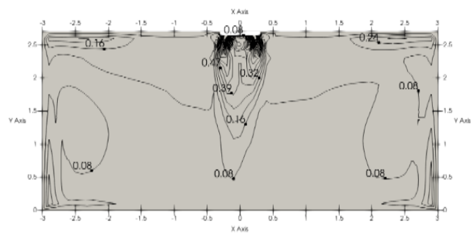
Figure 9.6: MIH36Q2HN18 heating at 300S
