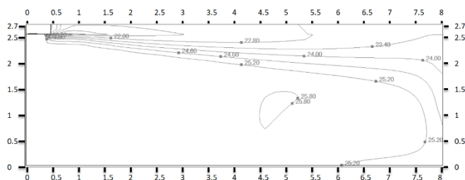
Figure 9.27: MIH71Q1HN18(A) cooling at 300S
