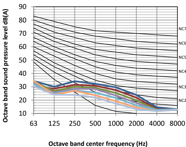
Figure 8.4: MIH28Q1HN18(A) octave band levels
