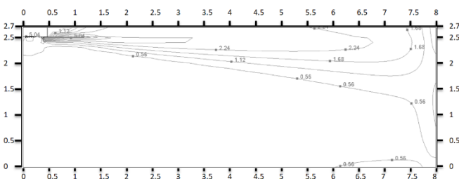
Figure 9.13: MIH71Q1HN18(A) cooling at 300S
