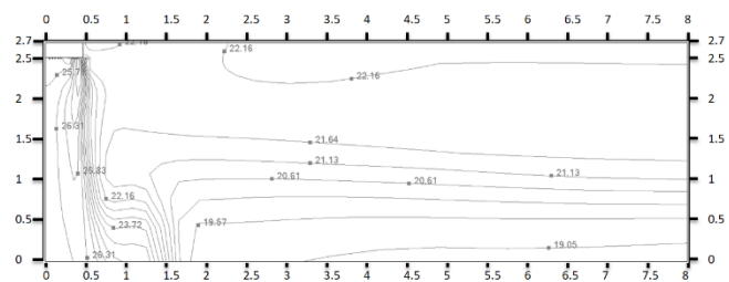
Figure 9.28: MIH71Q1HN18(A) heating at 300S
