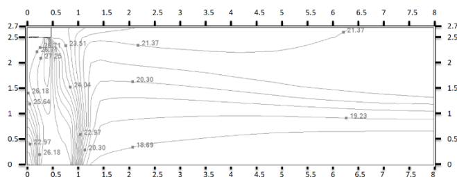
Figure 9.26: MIH56Q1HN18(A) heating at 300S
