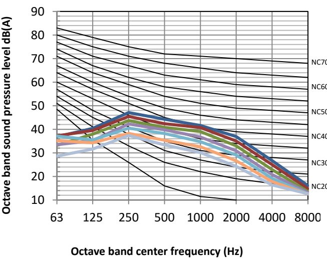
Figure 8.8: MIH71Q1HN18(A) octave band levels
