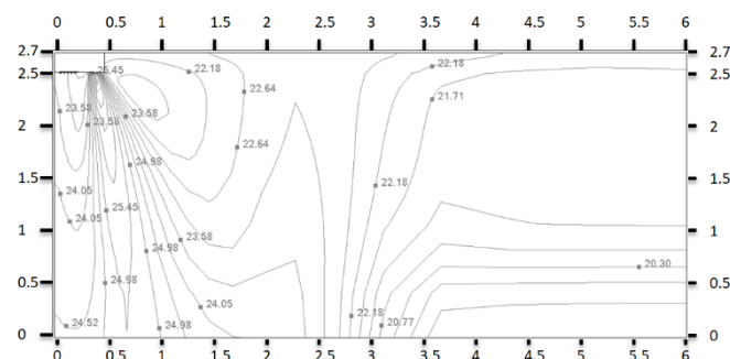
Figure 9.20: MIH28Q1HN18(A) heating at 300S
