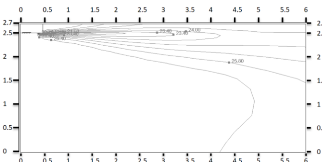
Figure 9.19: MIH28Q1HN18(A) cooling at 300S
