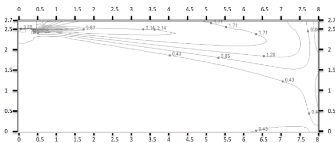
Figure 9.9: MIH45Q1HN18(A) cooling at 300S
