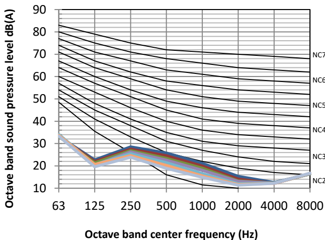
Figure 8.2: MIH18Q1HN18(A) octave band levels
