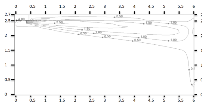
Figure 9.5: MIH28Q1HN18(A) cooling at 300S
