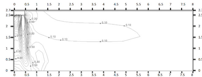
Figure 9.12: MIH56Q1HN18(A) heating at 300S
