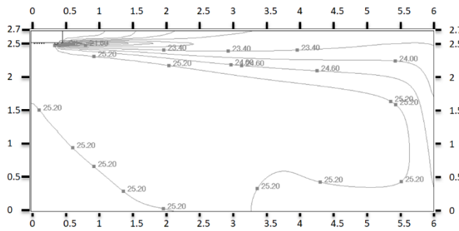
Figure 9.21: MIH36Q1HN18(A) cooling at 300S
