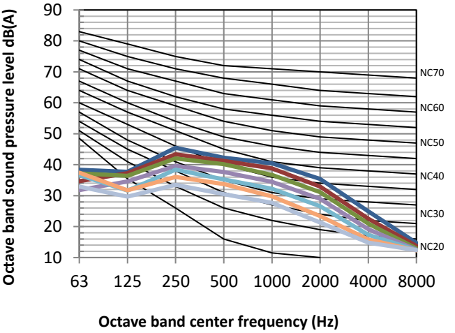
Figure 8.7: MIH56Q1HN18(A) octave band levels
