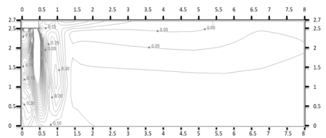
Figure 9.10: MIH45Q1HN18(A) heating at 300S
