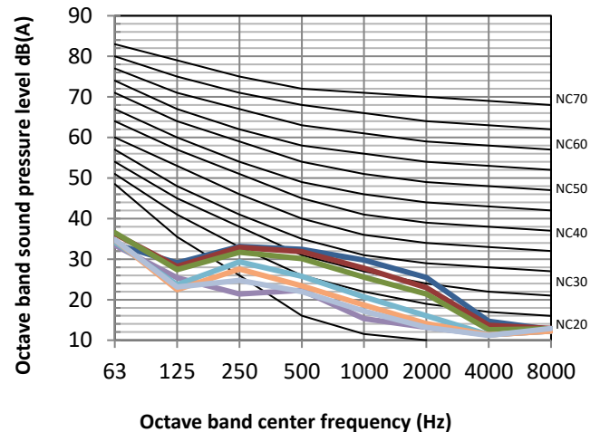
Figure 8.3: MIH22Q1HN18(A) octave band levels
