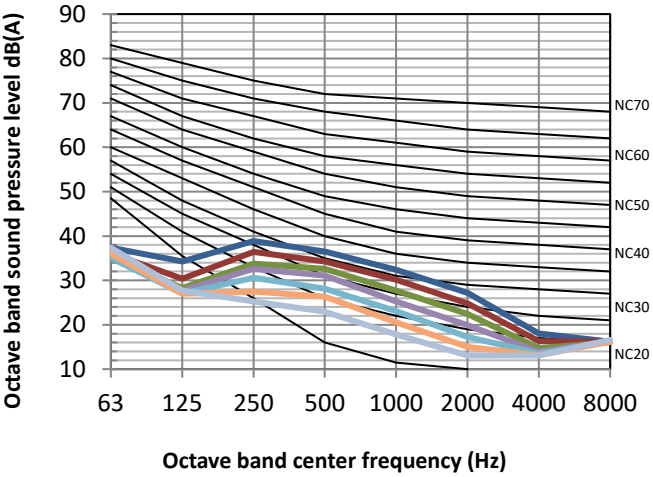
Figure 8.5: MIH45Q1HN18(A) octave band levels
