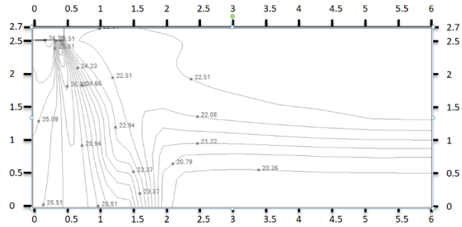
Figure 9.22: MIH36Q1HN18(A) heating at 300S
