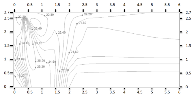
Figure 9.16: MIH18Q1HN18(A) heating at 300S
