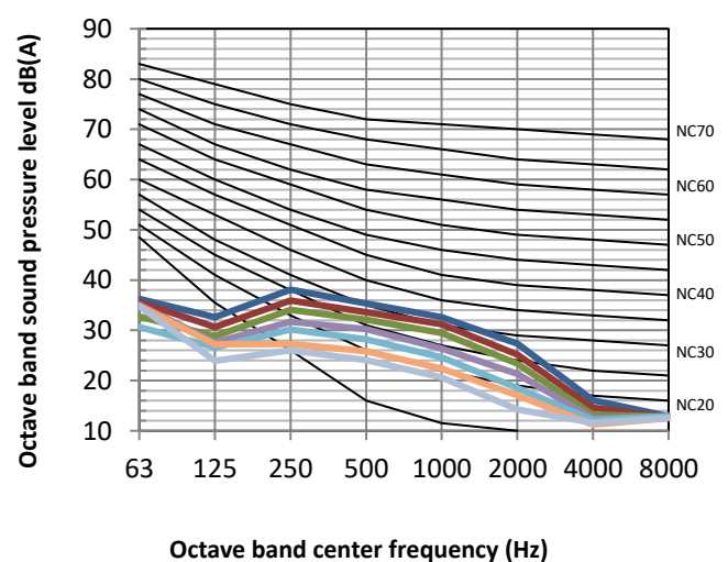
Figure 8.5: MIH36Q1HN18(A) octave band levels
