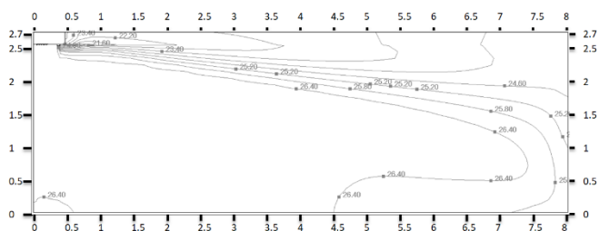
Figure 9.25: MIH56Q1HN18(A) cooling at 300S
