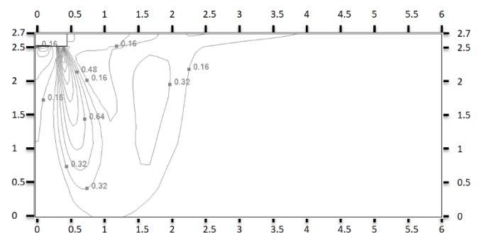
Figure 9.4: MIH22Q1HN18(A) heating at 300S
