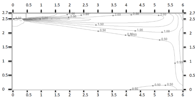
Figure 9.7: MIH36Q1HN18(A) cooling at 300S
