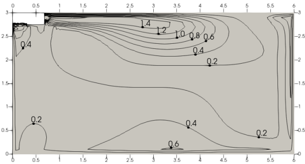
Figure 9.13: MIH100DLHN18 cooling at 300S
