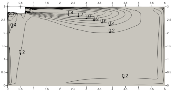
Figure 9.11: MIH90DLHN18 cooling at 300S
