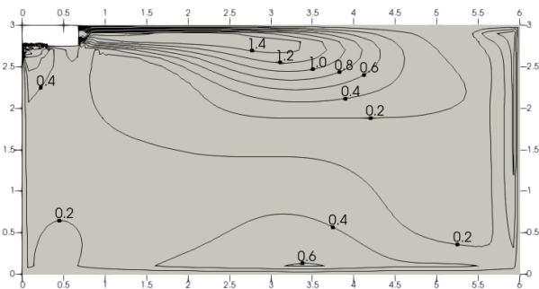
Figure 9.15: MIH112DLHN18 cooling at 300S
