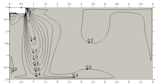
Figure 9.4: MIH45DLHN18 heating at 300S
