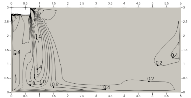
Figure 9.16: MIH112DLHN18 heating at 300S
