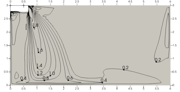
Figure 9.12: MIH90DLHN18 heating at 300S
