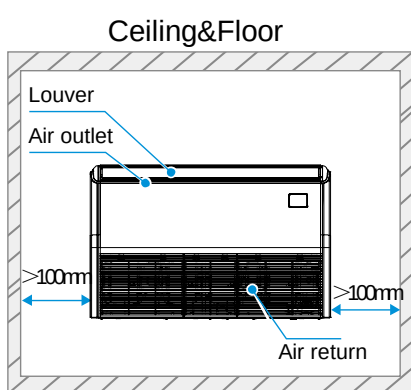
Figure 3.1: Ceiling & Floor space requirements (unit: mm)
